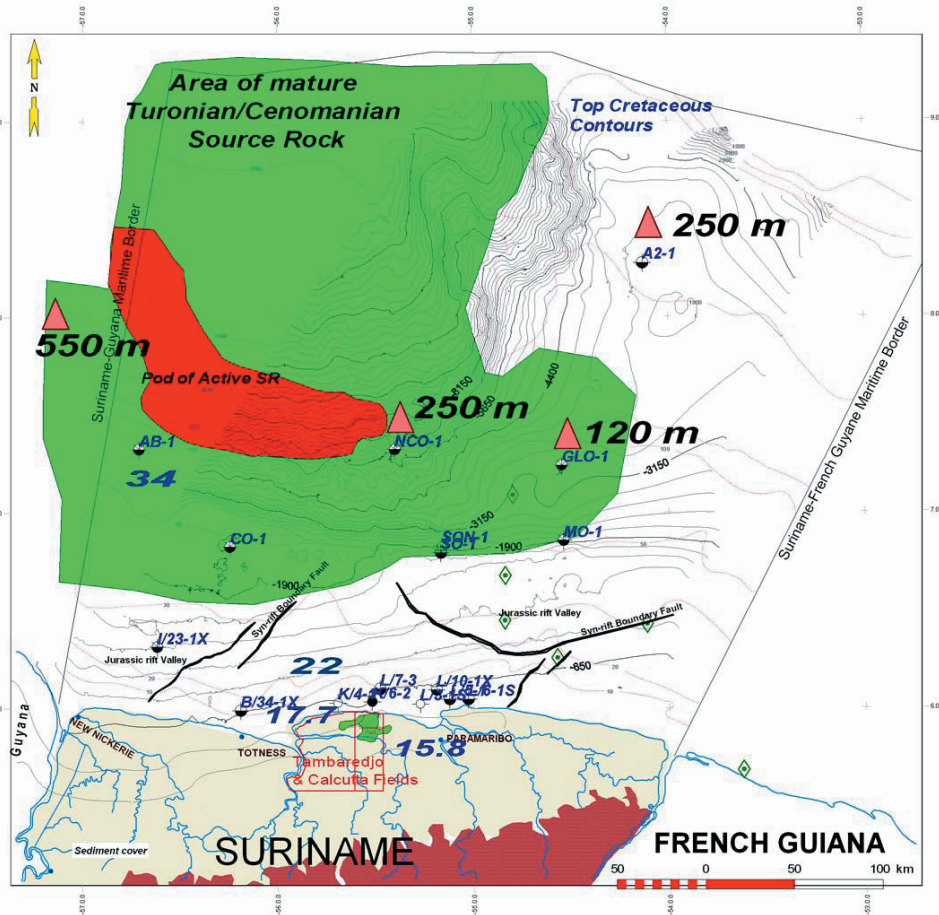
Figure 17: Cenomanian-Turonian Source Rock
