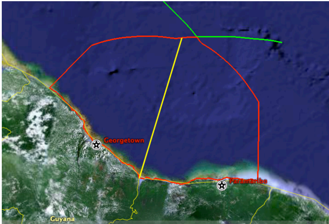
Figure 11. Division of the region shown in Figure 9 by the 17-degree line. The yellow line is a loxodrome with a bearing of 17 degrees. The green curves are extensions of the 200 nmi boundary.
